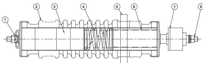
圖2 ZnO避雷器構造圖 (10kA) Fig.2 Structure of the ZnO lightning arrester (10kA)
