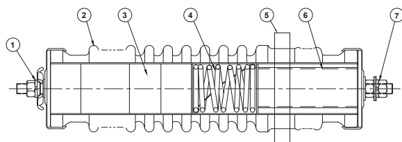
圖1 ZnO避雷器構造圖(5kA) Fig.1 Structure of the ZnO lightning arrester(5kA)
