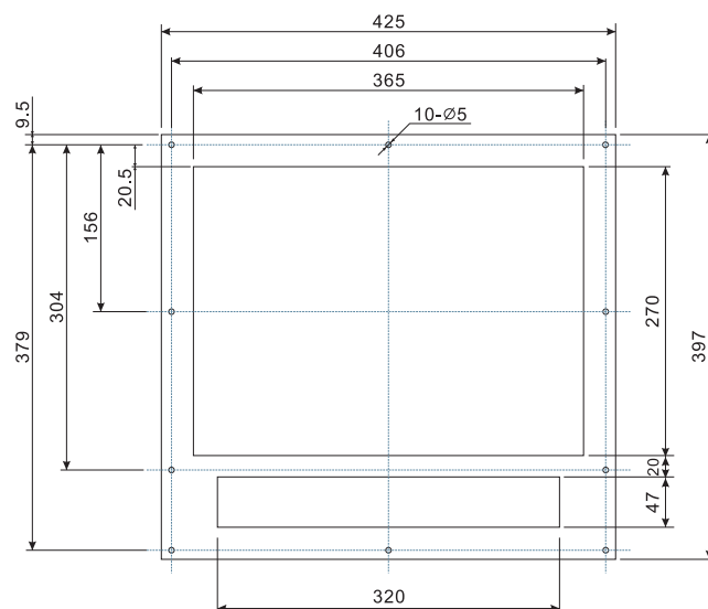
BA3200-H~BA6300-H抽出式門框(選購)
